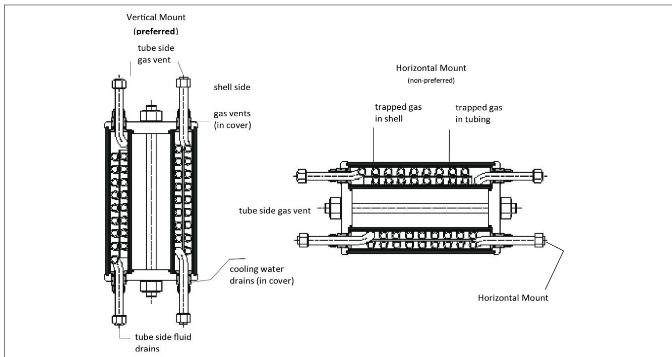
Figure 5: Cooler Mounting
